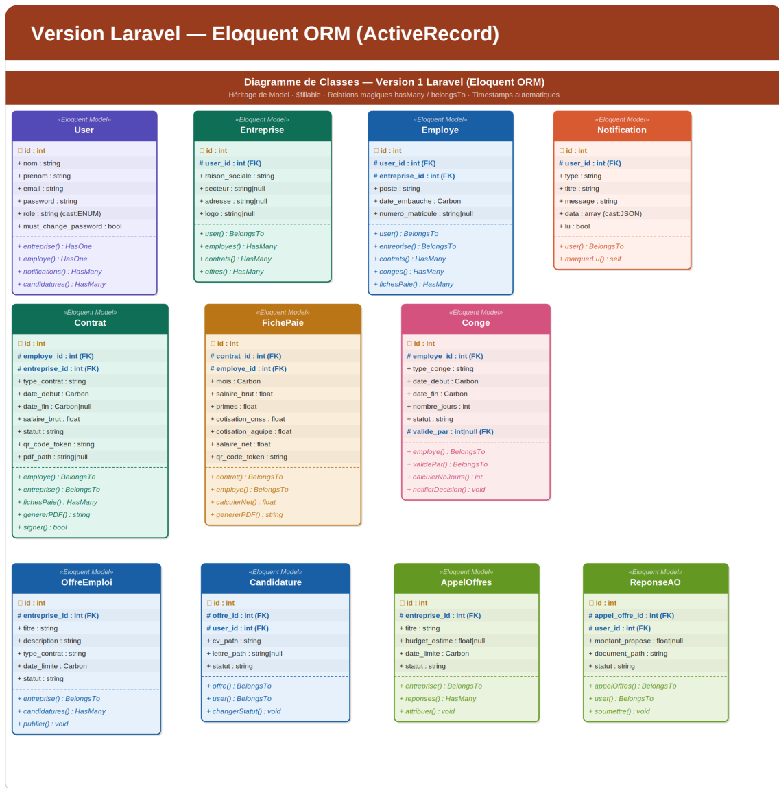
Figure 4a — Classes Laravel · Eloquent Model · 11 classes · hasMany/belongsTo · Facades
